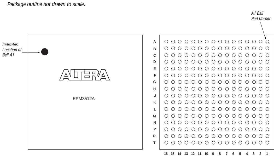
Figure 18. 256-Pin FineLine BGA Package Pin-Out Diagram
