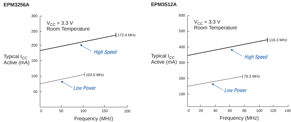
Figure 13. I_{CC} vs. Frequency for MAX 3000A Devices
