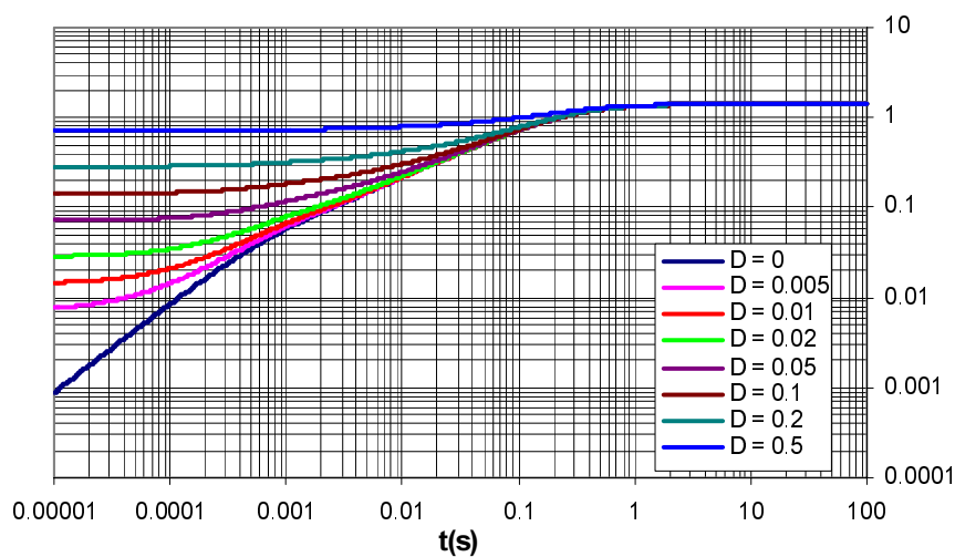
Transient thermal resistance junction to heatsink
