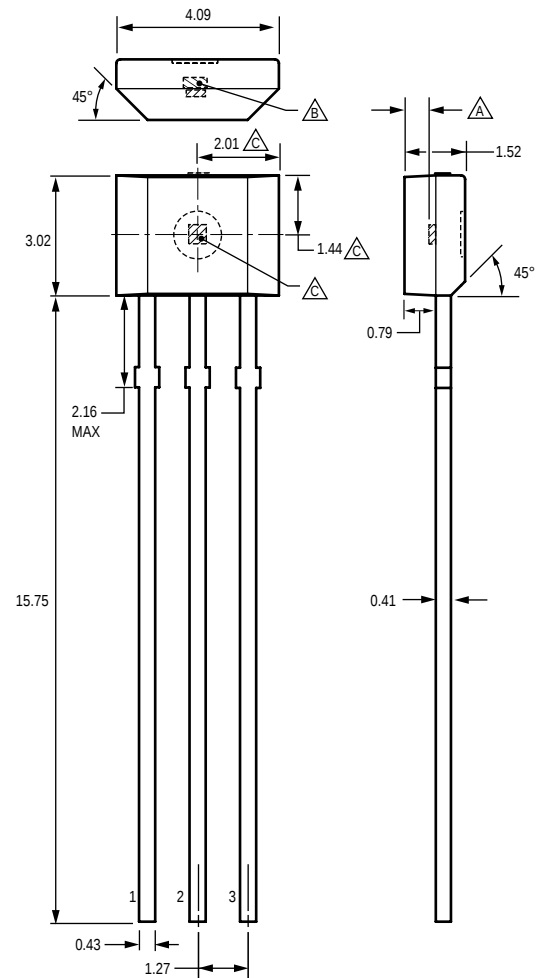
Package UA, Conventional Leadframe
