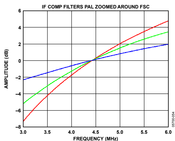
Figure 30. PAL IF Filter Compensation
