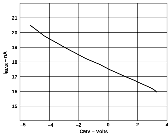
Figure 10. I_{BIAS} vs. CMV, V_S = \pm 5\text{ V}
