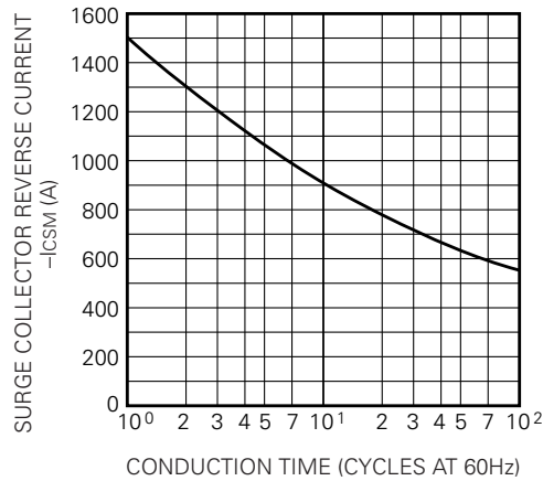
RATED SURGE COLLECTOR REVERSE CURRENT (DIODE FORWARD CURRENT)
