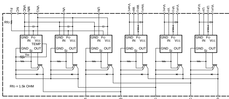
Outline Drawing and Circuit Diagram
