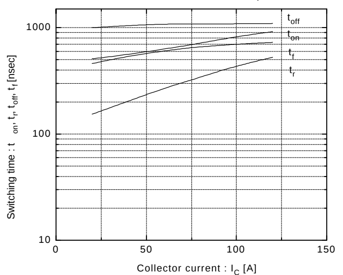
Switching time vs. Collector current V_{CC} = 600V, R_G = 16\Omega, V_{GE} = \pm 15V, T_J = 125^\circ\text{C}
