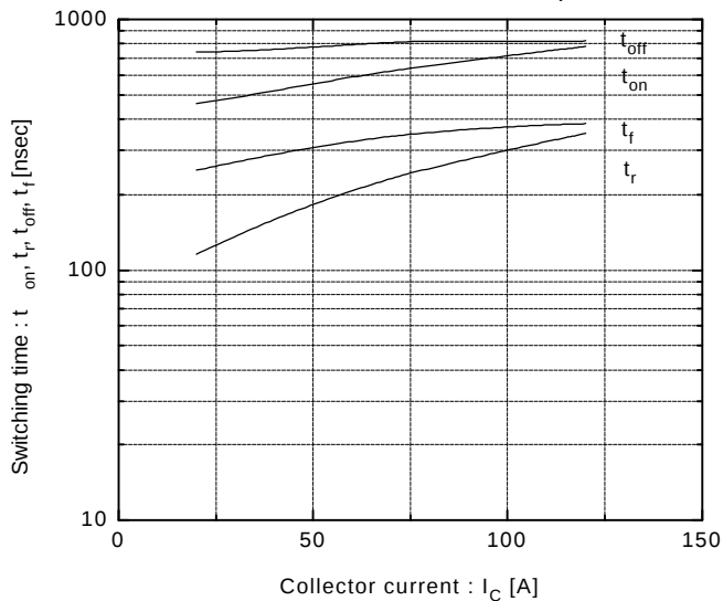
Switching time vs. Collector current V_{CC} = 600V, R_G = 16\Omega, V_{GE} = \pm 15V, T_J = 25^\circ\text{C}
