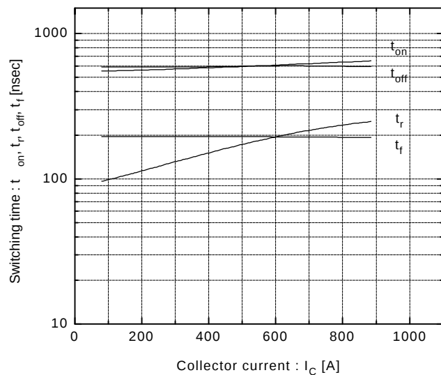
Switching time vs. Collector current V_{CC} = 300V, R_G = 2.7\Omega, V_{GE} = \pm 15V, T_J = 25^\circ\text{C}
