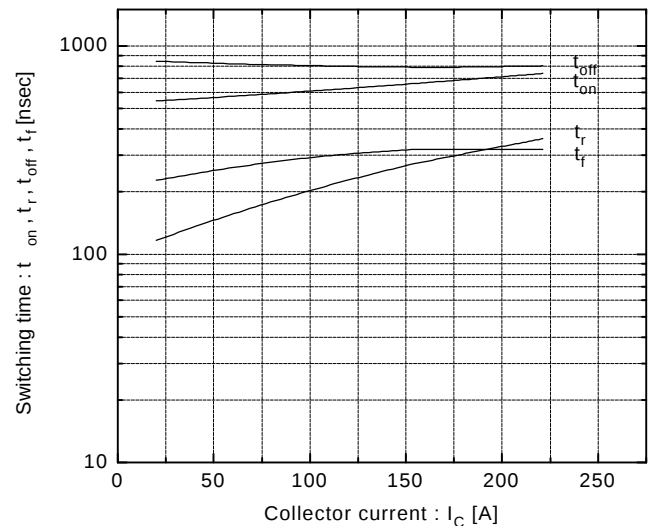
Switching time vs. Collector current V_{CC}=300V, R_G=16\Omega, V_{GE}=\pm 15V, T_J=125^{\circ}\text{C}
