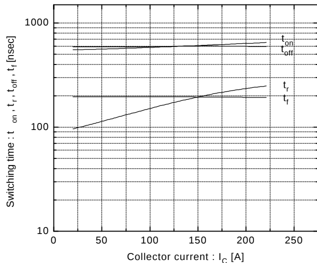
Switching time vs. Collector current V_{CC}=300V, R_G=16\Omega, V_{GE}=\pm 15V, T_J=25^{\circ}\text{C}
