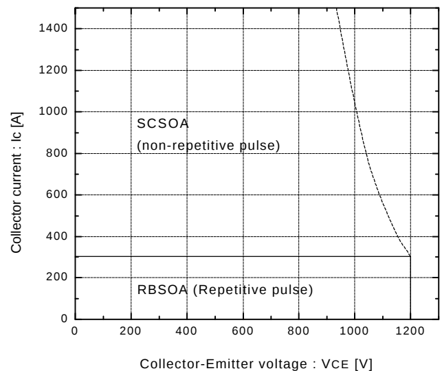
Reversed biased safe operating area +V_{GE}=15V , -V_{GE}\leq 15V , T_J\leq 125^\circ C , R_G\geq 5.6\Omega
