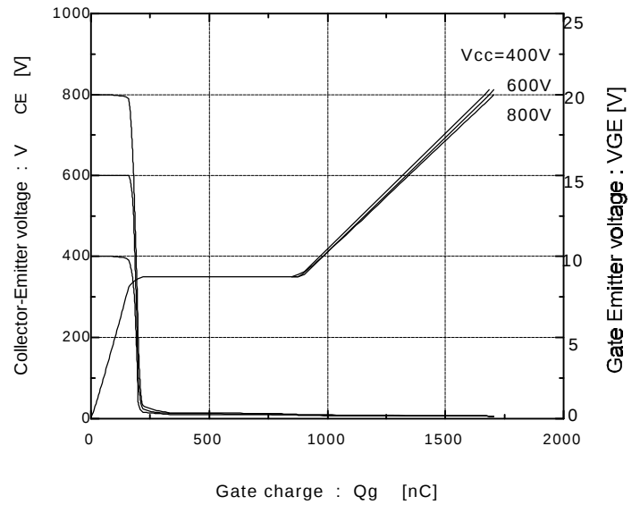
Dynamic input characteristics T_J=25^\circ C
