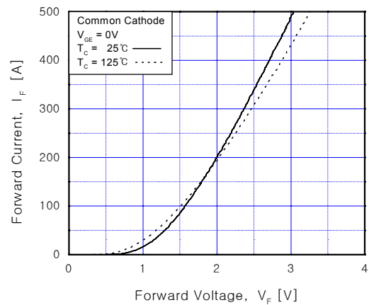
Fig 12. Forward Characteristics(diode)
