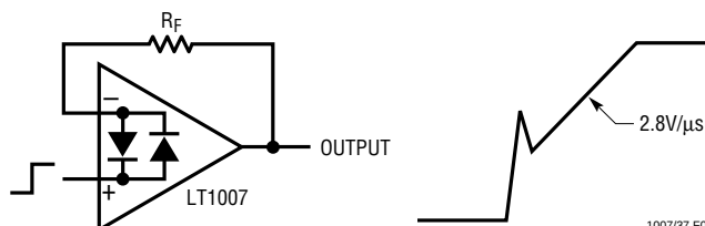
Figure 4. Pulsed Operation
