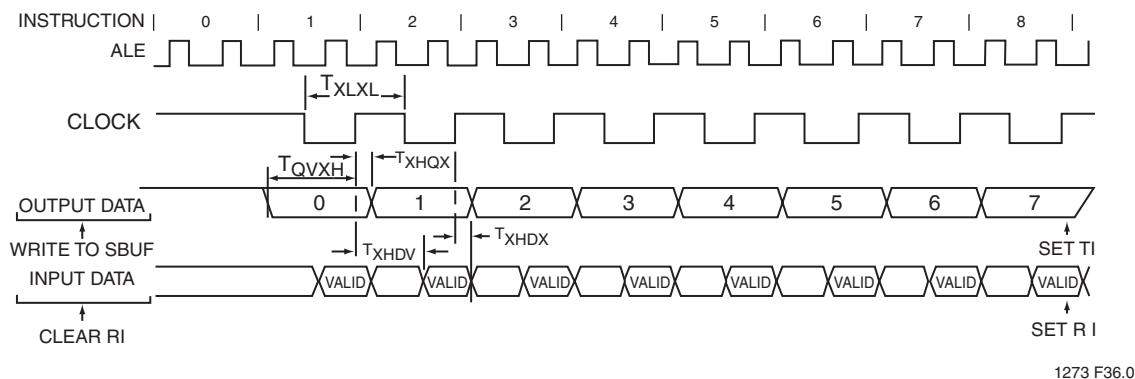
FIGURE 14-7: Shift Register Mode Timing Waveforms
