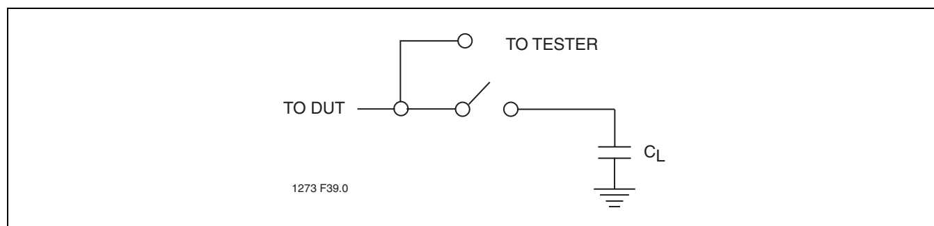
FIGURE 14-10: A Test Load Example
