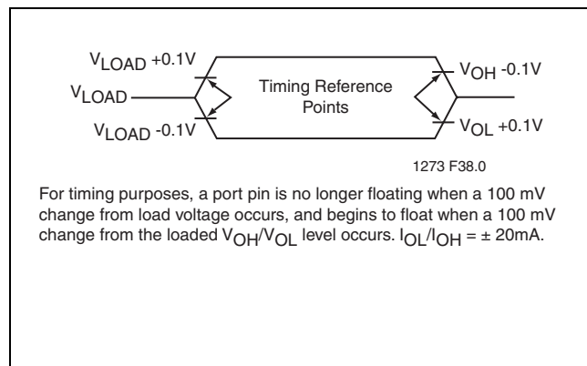
FIGURE 14-9: Float Waveform
