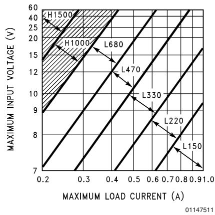
FIGURE 4. LM2575(HV)-5.0
