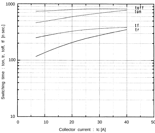
Switching time vs. Collector current V_{CC}=600\text{V} , R_G=51\text{ ohm} , V_{GE}=\pm 15\text{V} , T_J=25^{\circ}\text{C}
