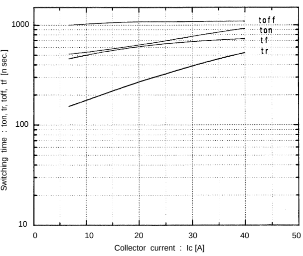
Switching time vs. Collector current V_{CC}=600\text{V} , R_G=51\text{ ohm} , V_{GE}=\pm 15\text{V} , T_J=125^{\circ}\text{C}
