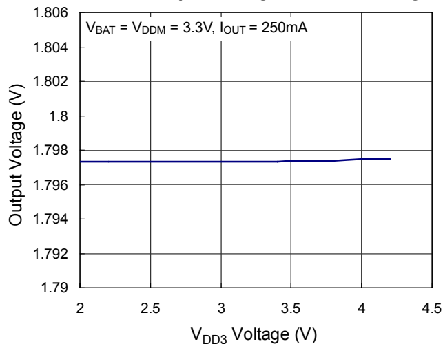
Buck3 Output Voltage vs. VDD3 Voltage
