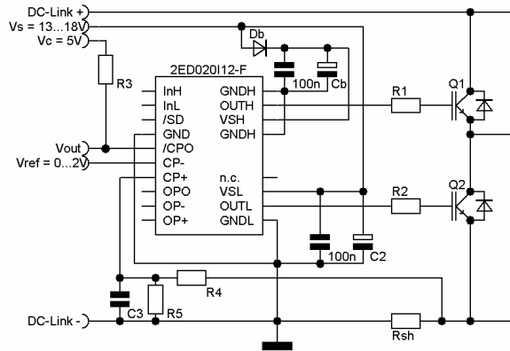
Figure 14 Over-current detection
