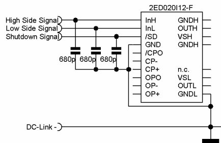
Figure 17 Logic inputs
