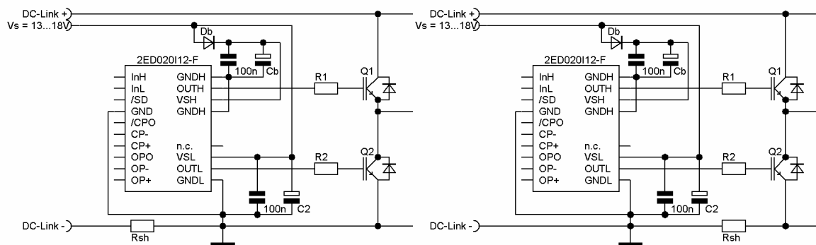
Figure 11 Ground reference
