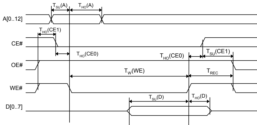
Figure 6: Write Cycle
