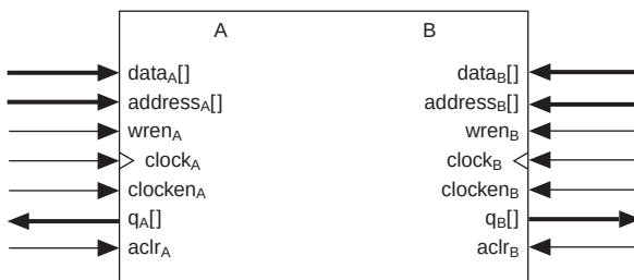
Figure 12. True Dual-Port Memory Configuration
