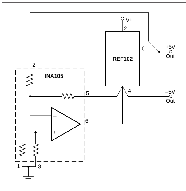
FIGURE 12. \pm 5\text{V} Reference.
