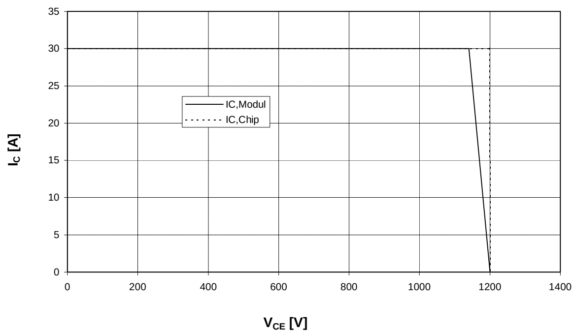
Reverse bias safe operating area Inverter (RBSOA) T_{vj} = 125^\circ C , V_{GE} = \pm 15V , R_G = 47 \text{ Ohm}
