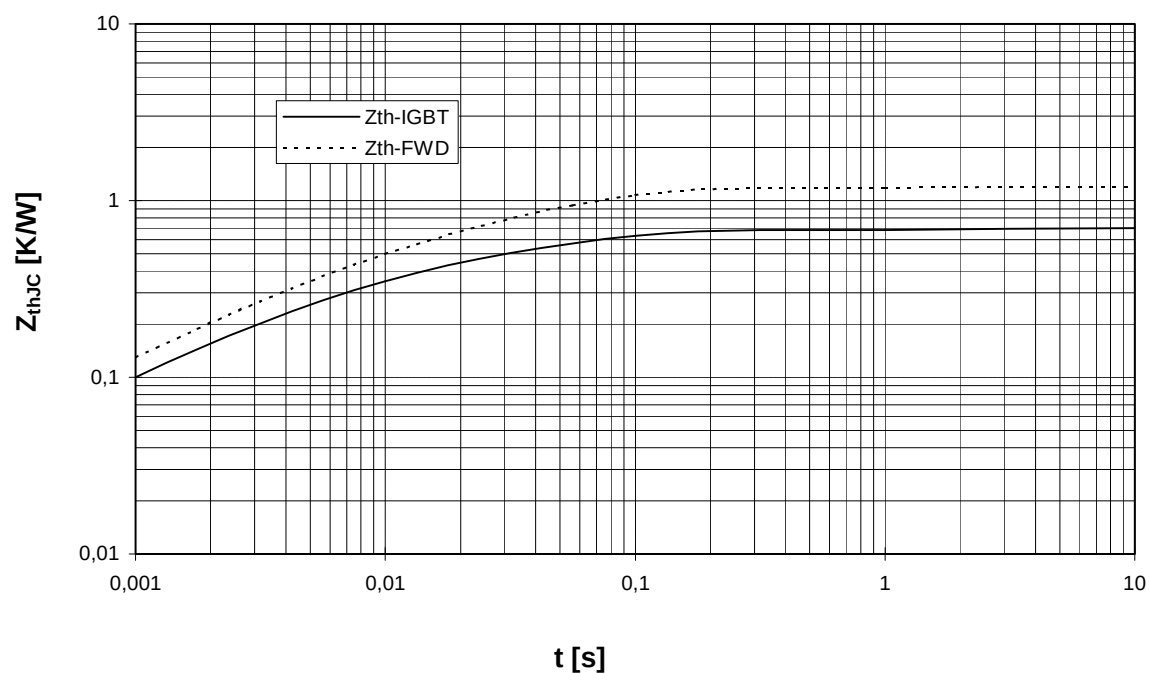
Transient thermal impedance Inverter
