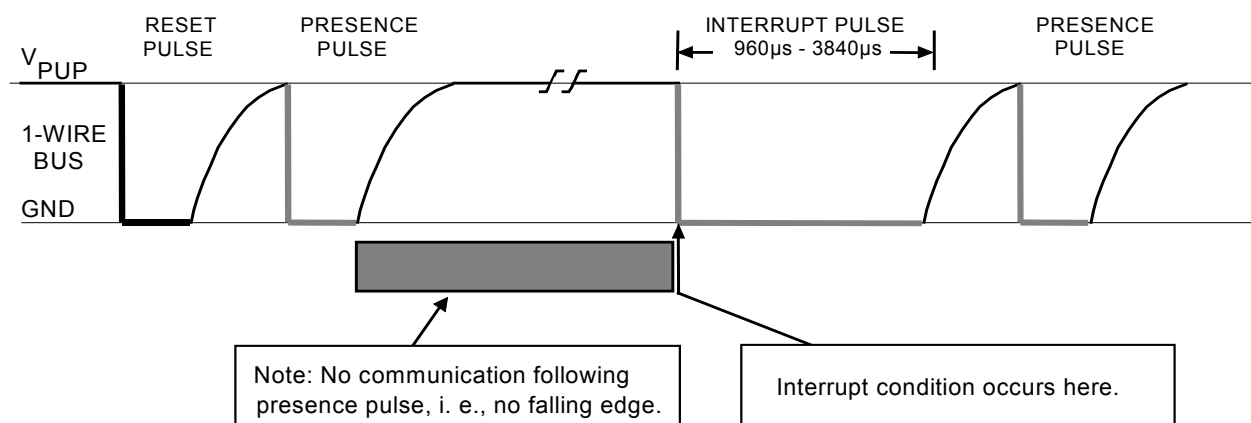
Figure 12. TYPE 1 INTERRUPT
