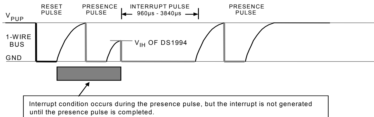
Figure 14. TYPE 2 INTERRUPT
