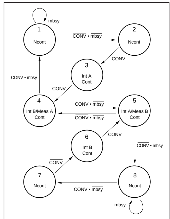
FIGURE 9. State Diagram.
