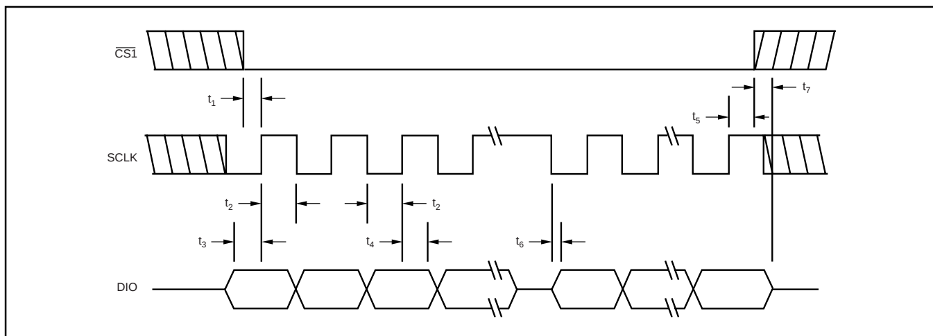
FIGURE 6. Timing Diagram for Writing to and Reading From the XTR108 with EEPROM Readback Disabled. (See Table XIV for timing key.)
