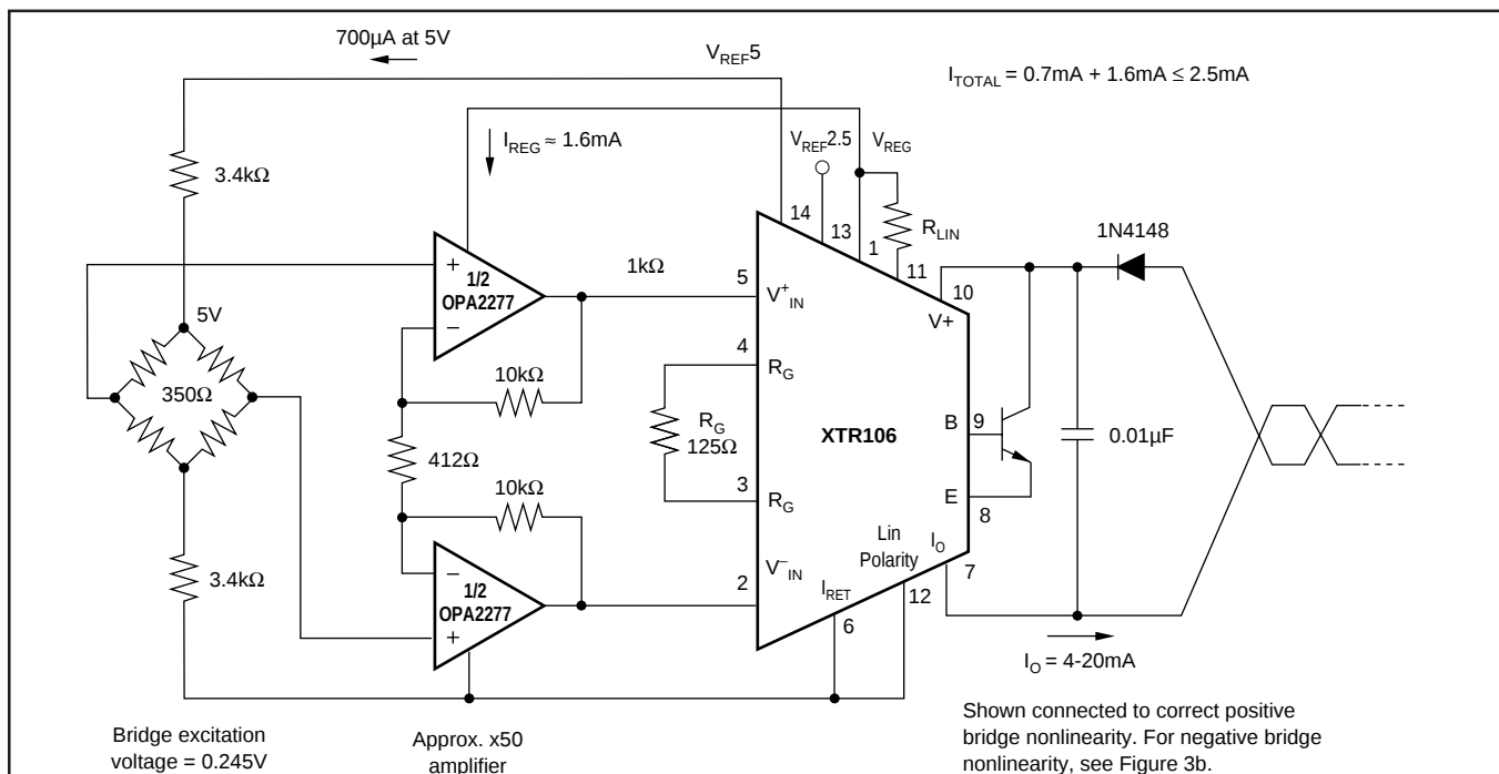
FIGURE 5. 350Ω Bridge with x50 Preamplifier.
