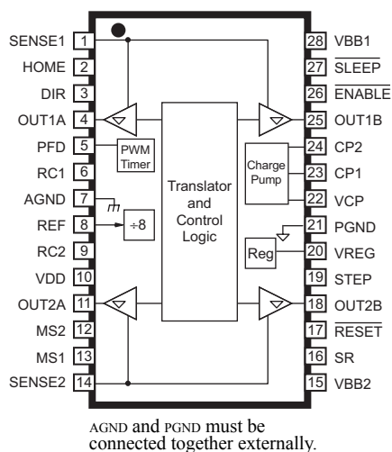
Package LP, 28-pin TSSOP with Exposed Thermal Pad
