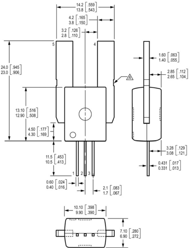
Package CB-PSS
