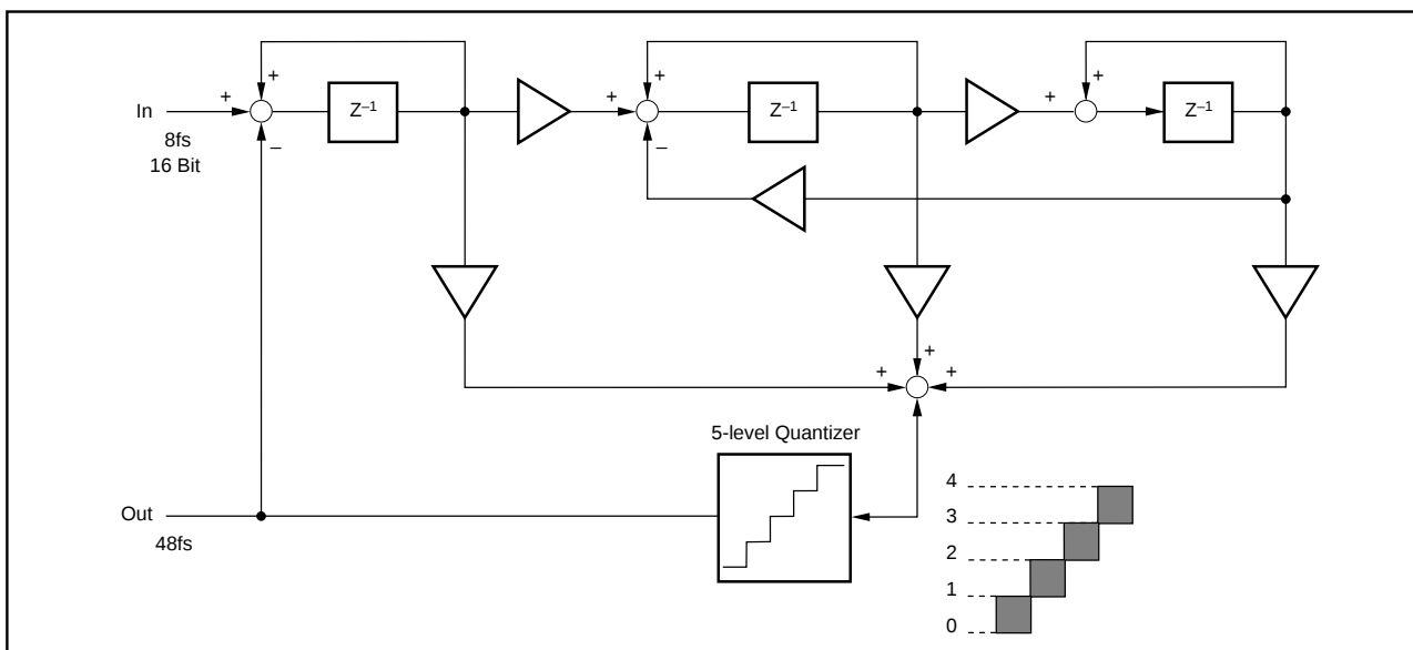
FIGURE 10. 5 Level \Delta\Sigma Modulator Block Diagram.
