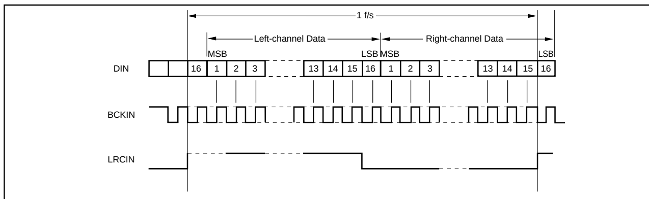
FIGURE 2 . IIS Format, 16-Bit (32 BCKIN/fs, continuous data).
