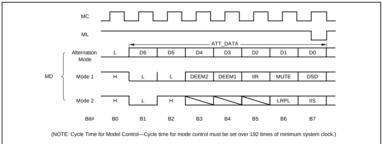
FIGURE 5. Mode Control Input Format, Serial Mode.
