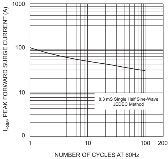
Fig. 6 Peak Forward Surge Current vs. Number of Cycles at 60Hz
