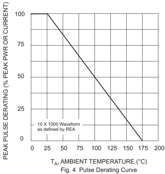
Fig. 4 Pulse Derating Curve
