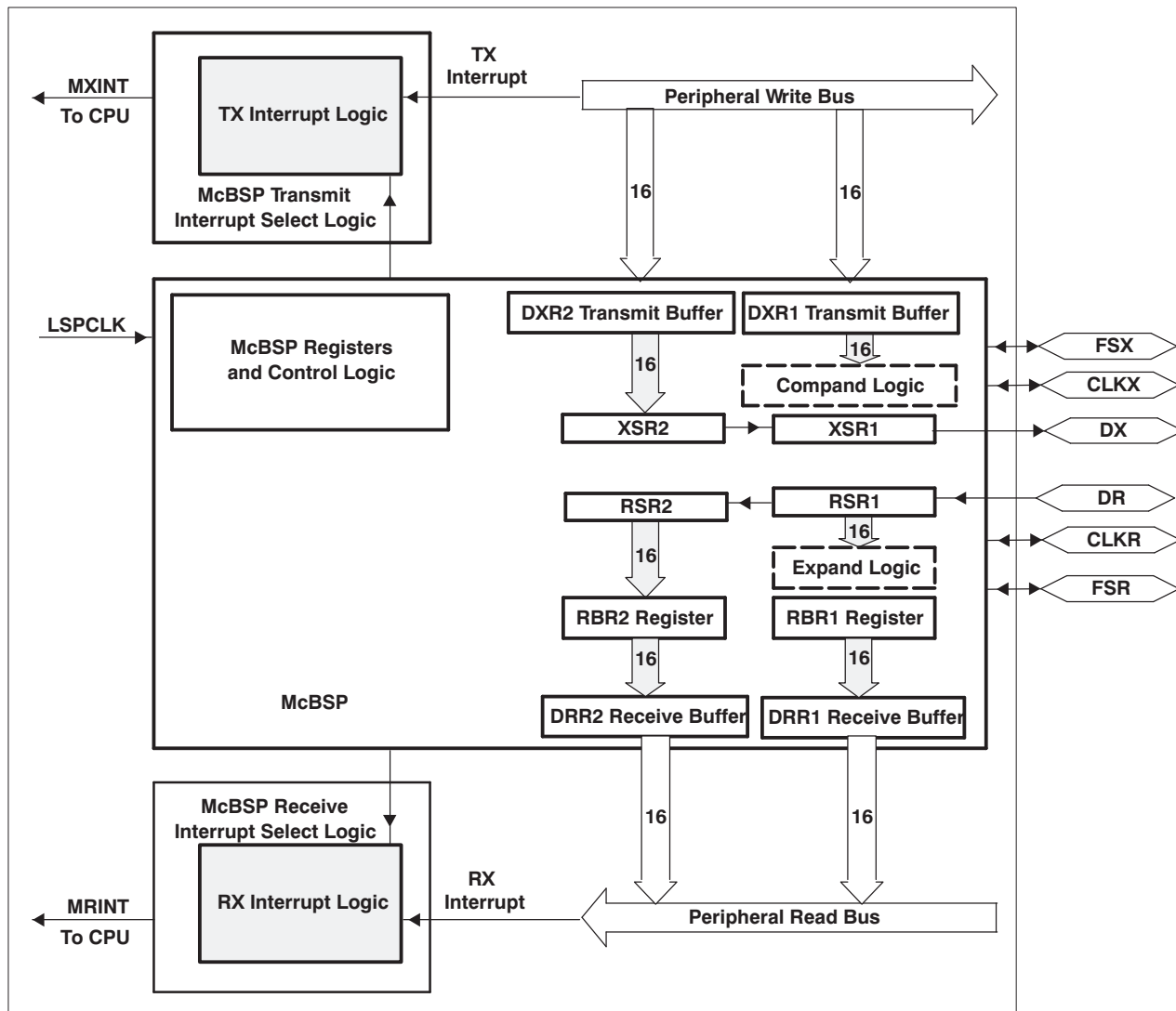
Figure 4-11. McBSP Module
