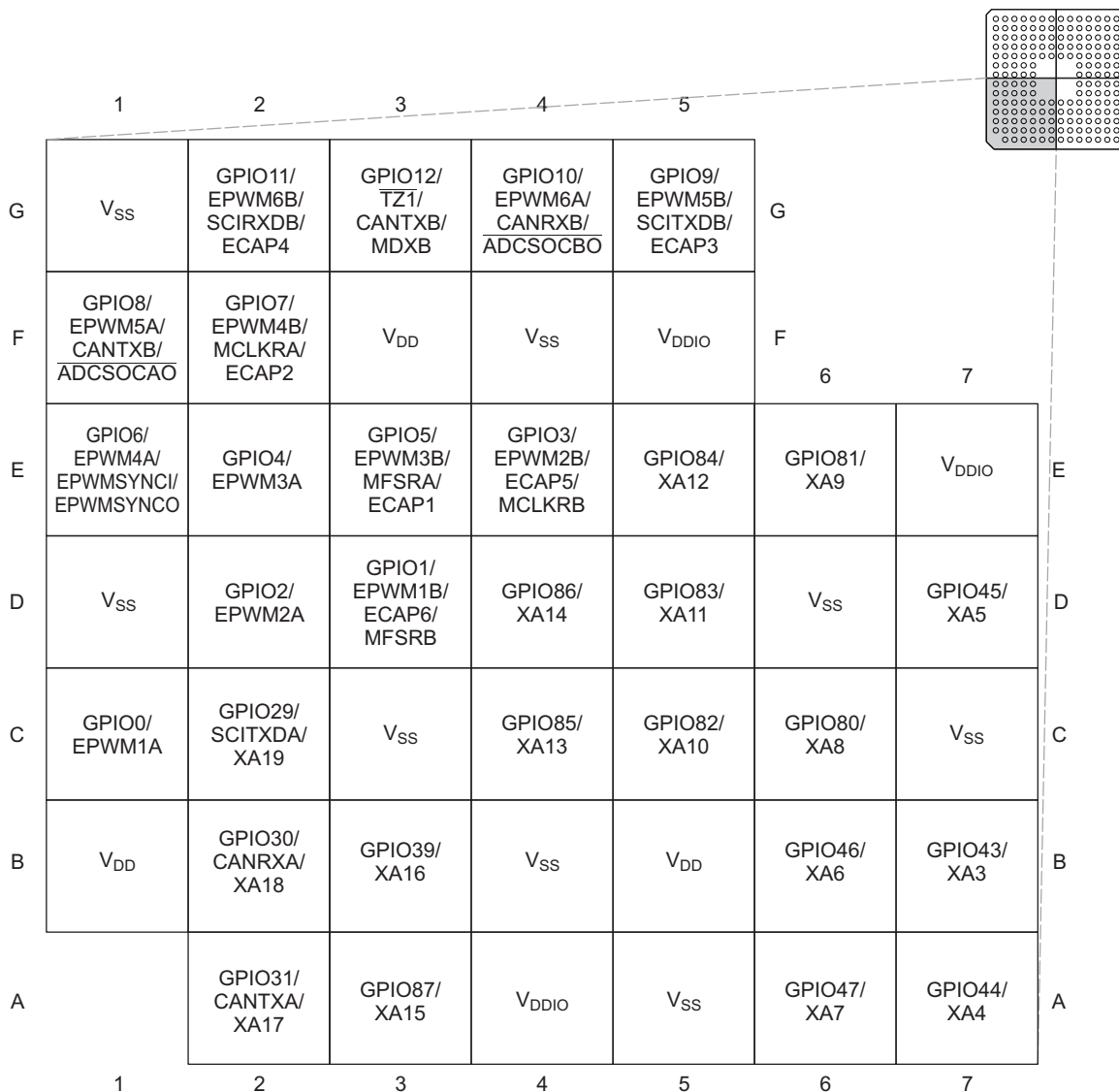
Figure 2-4. F28335, F28334, F28332 179-Ball ZHH MicroStar BGA™ (Lower Left Quadrant) (Bottom View)
