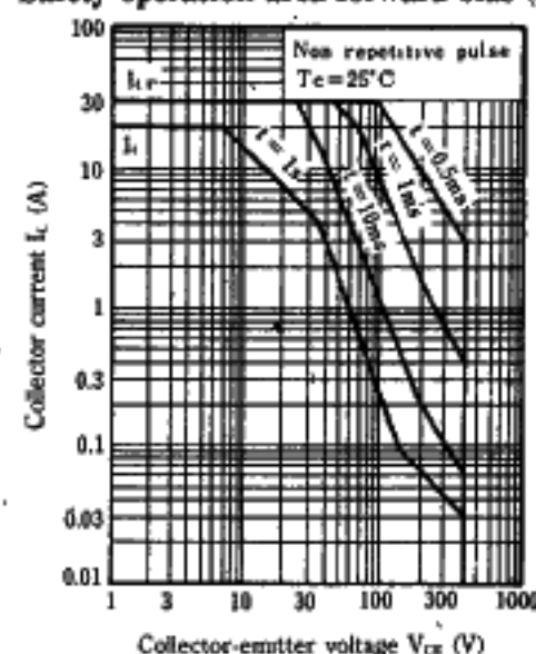
Safety operation area-forward bias (ASO)
