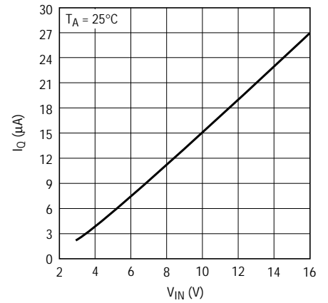
Shutdown Quiescent Current ( I_Q at CTRL = 0V )
