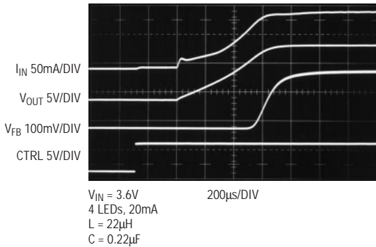
Figure 5. Start-Up Waveforms
