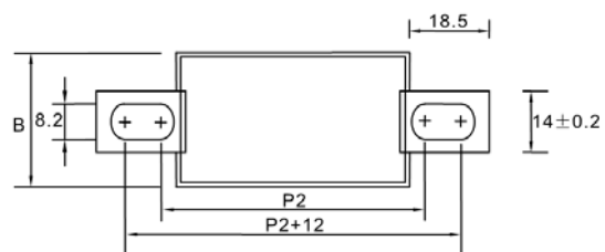
Fixing pitch and distance between lugs: Style E
