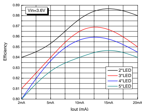
Figure 2. Efficiency vs Number of LEDs
