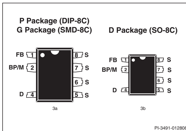
Figure 3. Pin Configuration.
