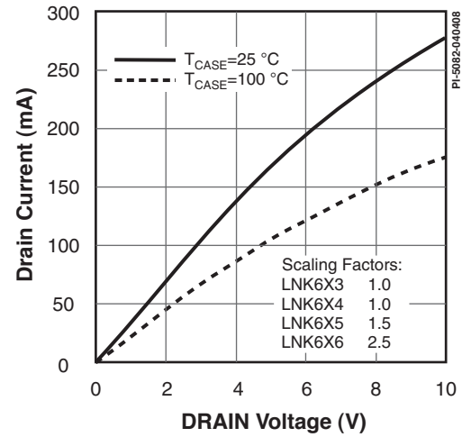
Figure 16. Output Characteristic.
