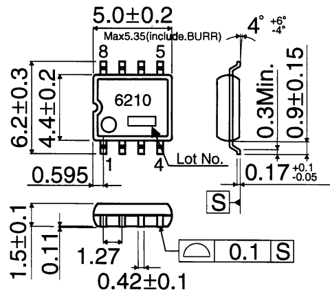
SOP8 (Unit: [mm])
